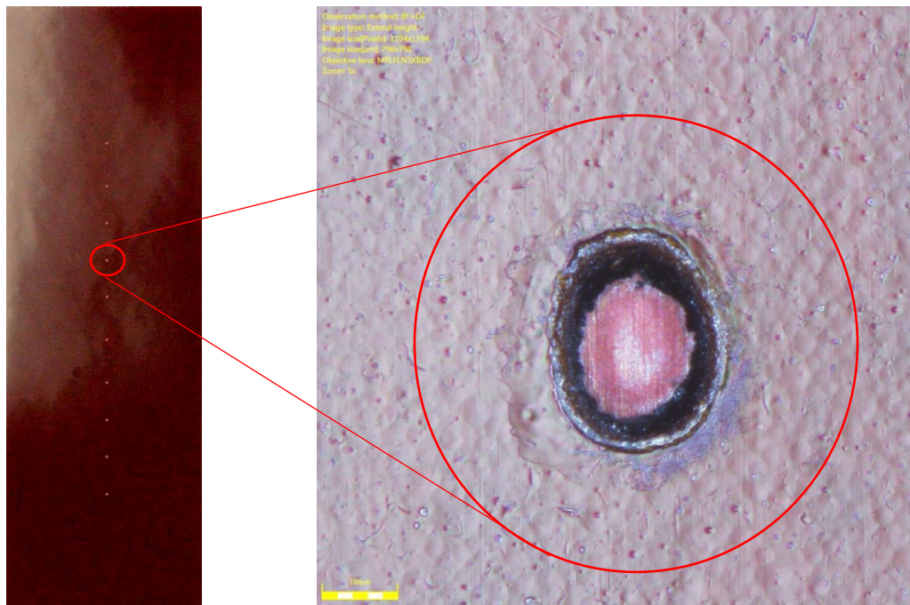
Figure 2. Ten vias through polyimide layer (left); Close up of an individual via revealing clean removal of polyimide to expose underlying copper (right).
